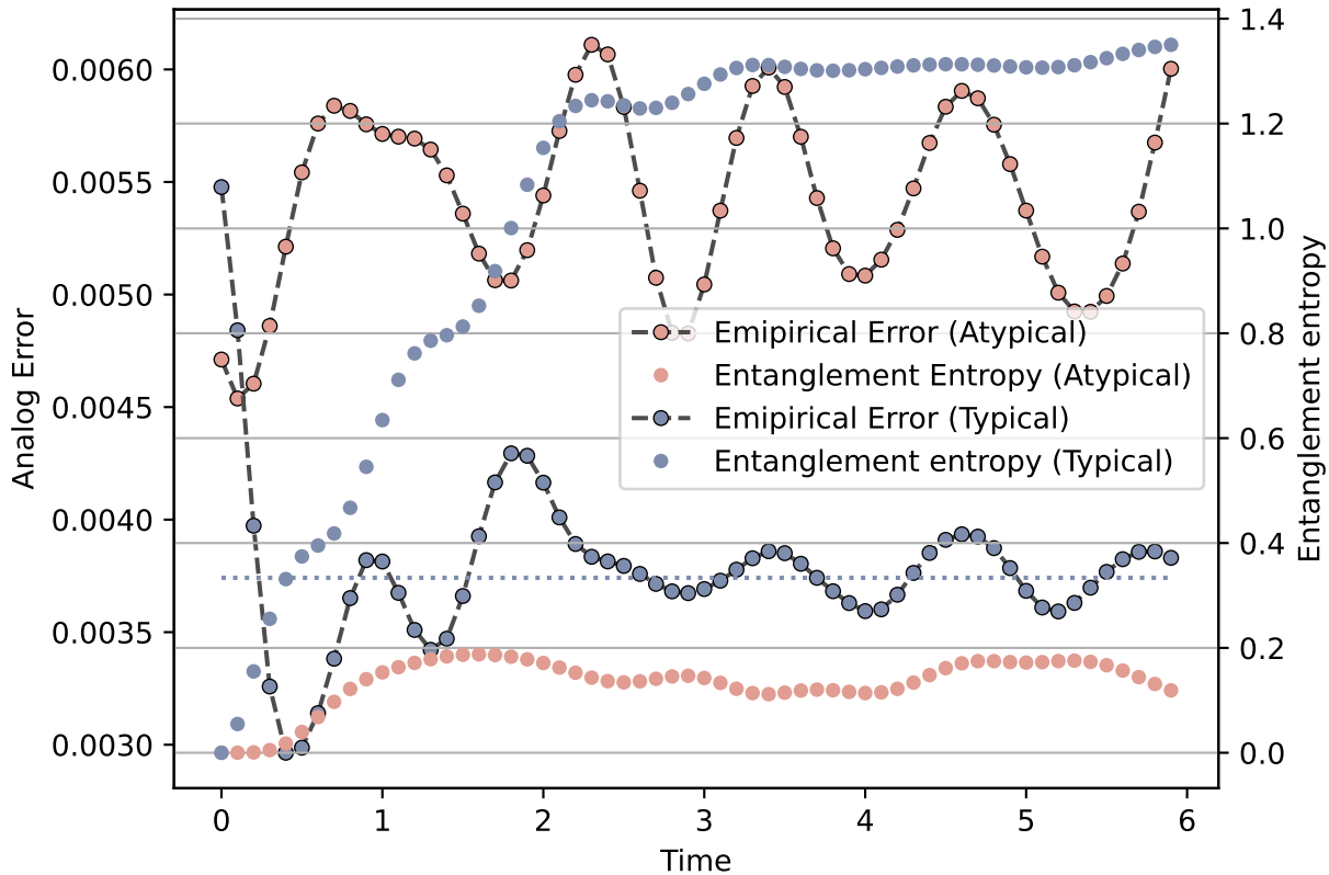
QIMF, one segment evolution with disorder
